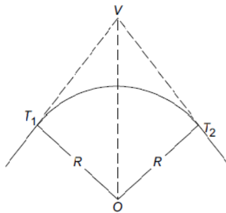
Fig: Simple Circular Curve
