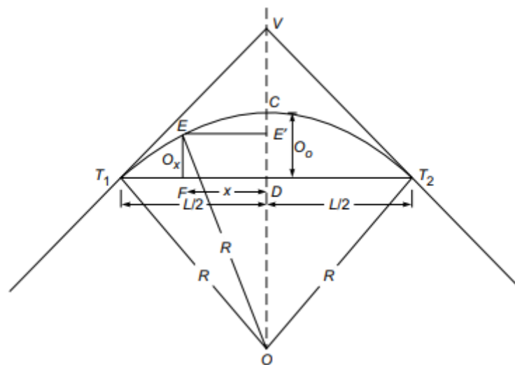
Fig: Offset from long chord
