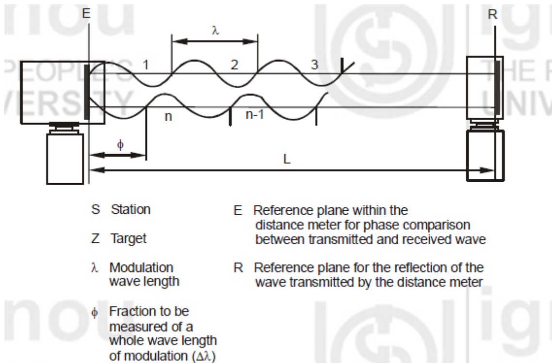
Fig : Principle of EDM Measurement
