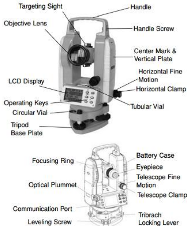
Fig: Parts of a Theodolite
