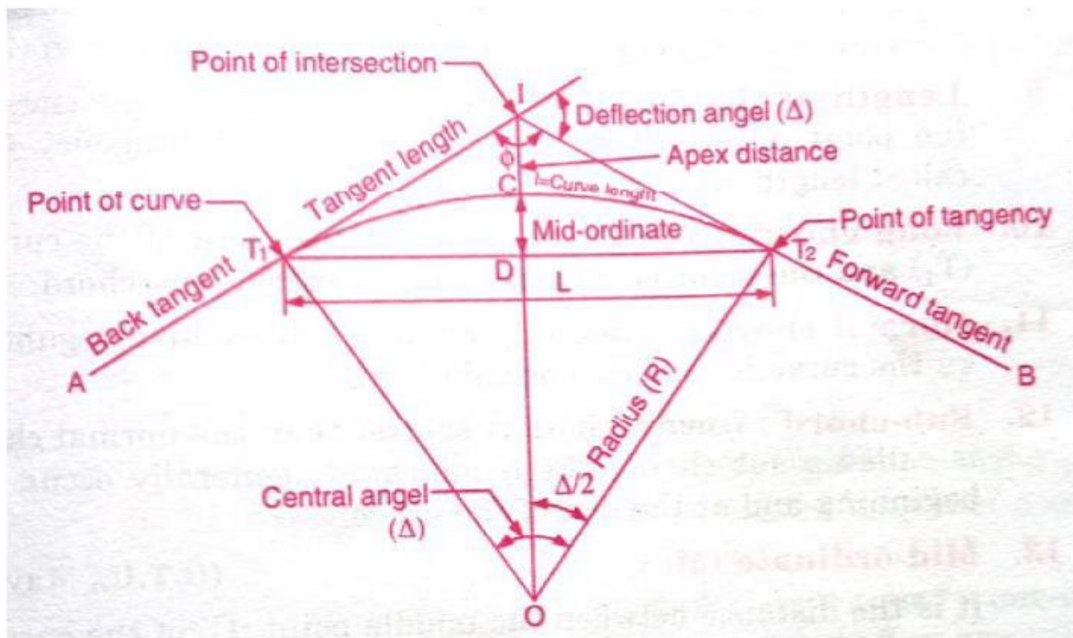
Fig: Elements of Simple Curve
