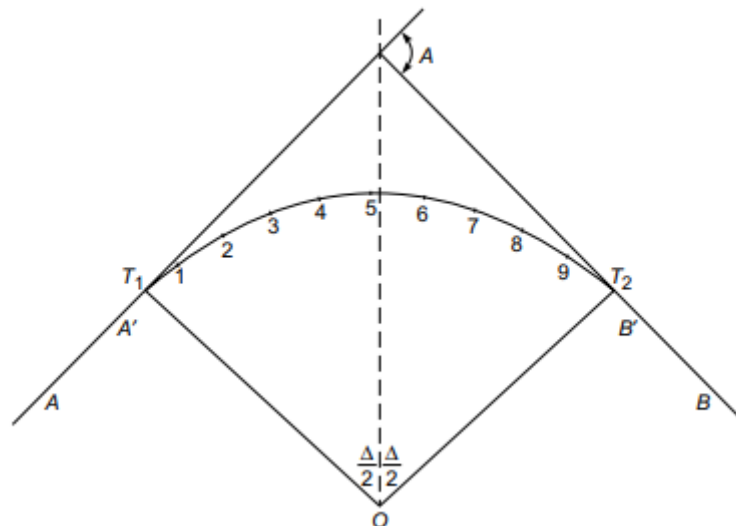
Fig: Setting out of Simple Circular Curve
