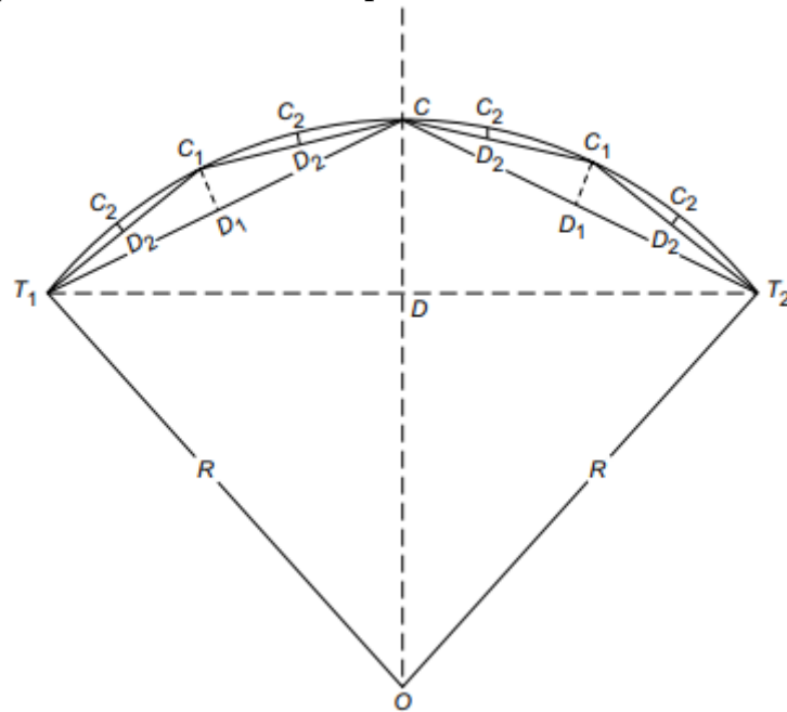
Fig: Successive bisection of chord
