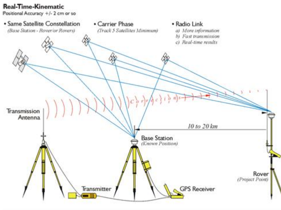
Fig.—RTK GPS basic concept
