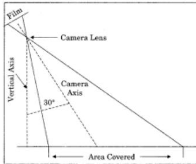
Fig. Low Oblique Photograph
