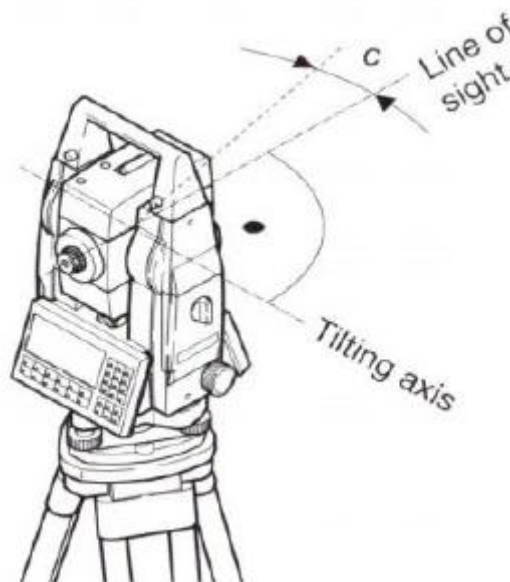
Fig.: Collimation errors
