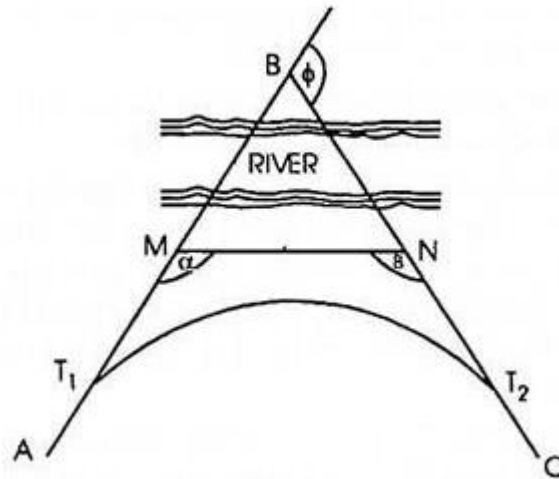
Fig: Point of Intersection is Inaccessible
