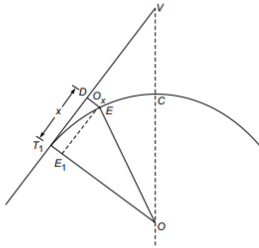
Fig: Perpendicular Offset Method
